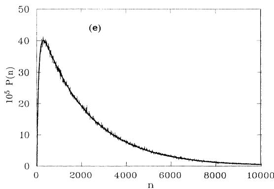
FIG. 3. The probability P(n) to leave the interval [x_{th}, \infty] for the first time after n time steps from N = 5 \times 10^5 numerical realizations of the Langevin equation (2.1) with initial condition x_0 = x_s . The map f(x) is given by the example of Fig. 2. The threshold x_{th} is chosen at x_{th} = -L - 1 . The bold curves represent the theoretical predictions (3.21) and (4.4)–(4.6) of the Markovian three-state model. The parameter values are (a) u = 5 , \epsilon = 0.18 , and L = 100 ; (b) u = 5 , \epsilon = 0.18 , and L = 20 ; (c) u = 5 , \epsilon = 0.24 , and L = 500 ; (d) u = 4.8 , \epsilon = 0.2 , and L = 17 ; and (e) u = 5.05 , \epsilon = 0.2 , and L = 71 . Thus for (a), (d), and (e) k \approx k_+ \approx 10^{-3} ; (b) 10^{-2} \approx k_+ \ll k \approx 10^{-3} ; and (c) 10^{-2} \approx k \ll k_+ \approx 10^{-3} , according to Eqs. (3.21) and (4.6). The very small values of the numerical P(n) for the first few n are an initial effect similar to the behavior shown in Fig. 1. The differences of the numerical and theoretical results are of the same order as the respective errors of the rates k and k_+ at the same parameter values. In (d), the thin curve represents P(n) given by (4.4) and (4.5) but with fitted rates k and k_+ , thus indicating the excellent agreement of the simulations with the Markovian three-state model. In the other cases (a)–(c) and (e), such a fitted model cannot be distinguished from the theoretical results.
